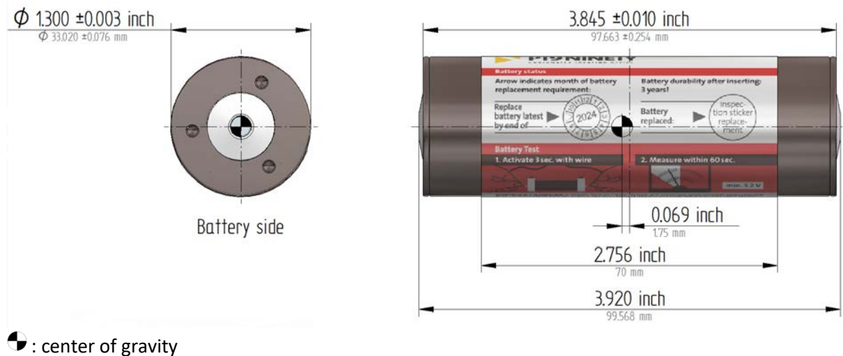
Figure 3: ULD Dimensions
