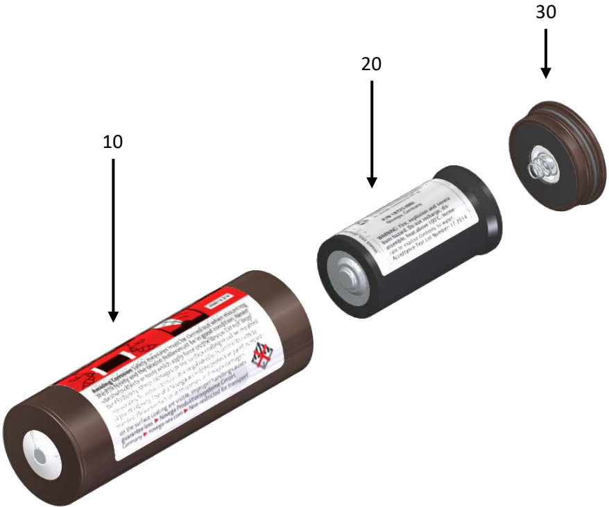
Figure 9: Illustrated Parts
